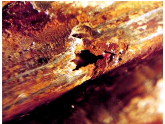
Example of damage to water supply piping in a large brewery - SS type 316L with a diameter of almost one metre.
